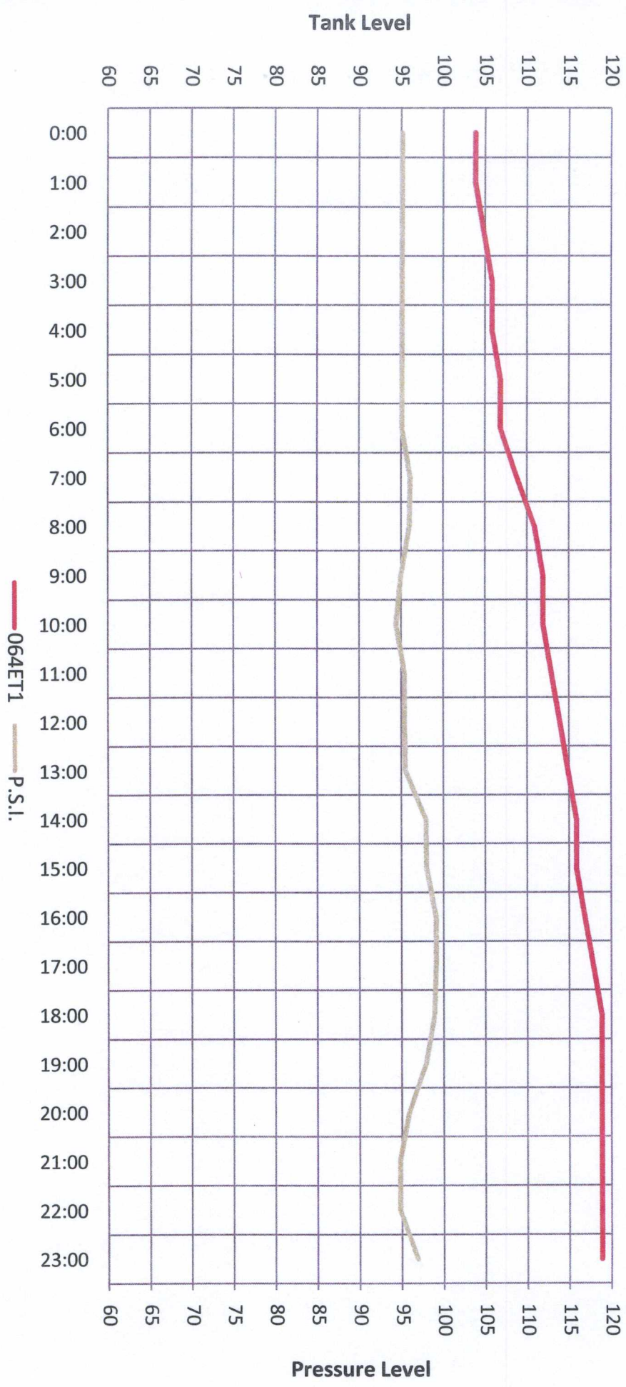
Facility 064 Elevated Tank & Pressure Levels August 22, 2009
